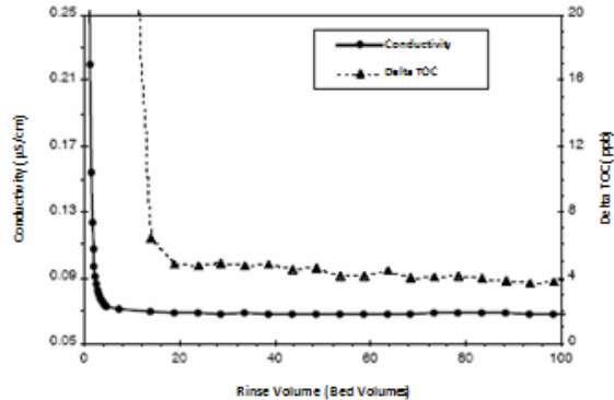
Figure 3: Conductivity and TOC Rinse-down
